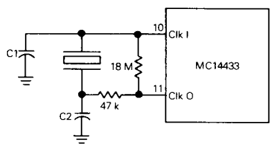
(a) Crystal Oscillator Circuit
