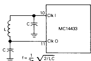
(b) LC Oscillator Circuit
