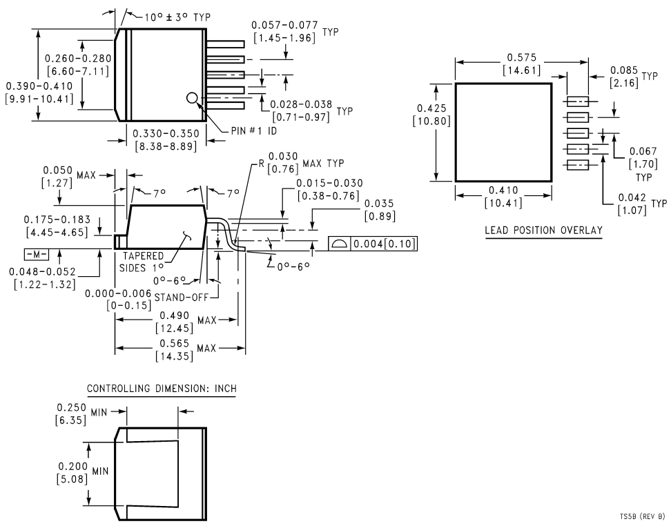
5-Lead TO-263 (S) Order Number LM2577S-12, LM2577S-15 or LM2577S-ADJ NS Package Number TSS5B
