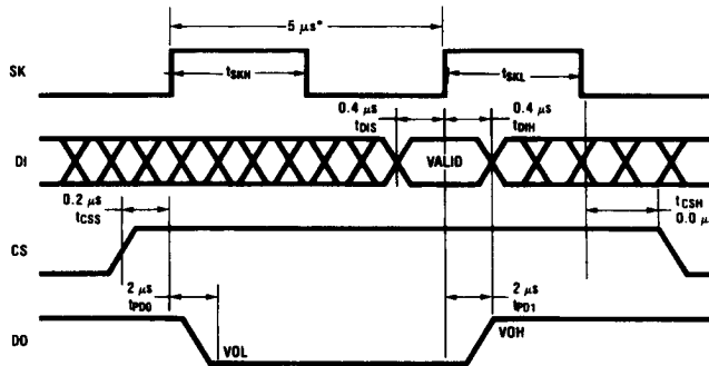
Synchronous Data Timing
