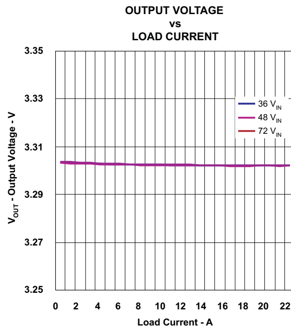
Figure 4. Load Regulation
