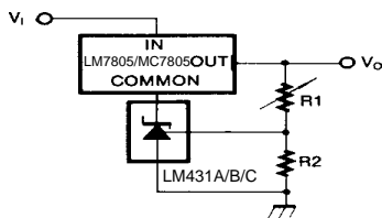
Figure 12. Output Control for Three-Termi- ninal Fixed Regulator
