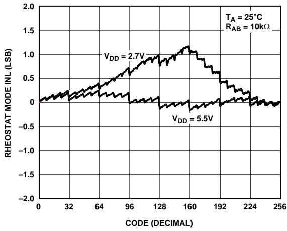
Figure 2. R-INL vs. Code vs. Supply Voltages
