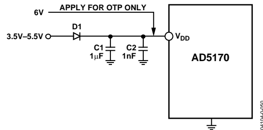
Figure 38. Isolate 6 V OTP Supply from 3.5 V to 5.5 V Normal Operating Supply. The 6 V supply must be removed once OTP is completed.
