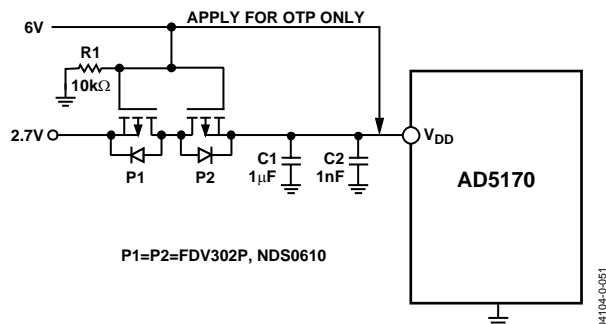
Figure 39. Isolate 6 V OTP Supply from 2.7 V Normal Operating Supply. The 6 V supply must be removed once OTP is completed
