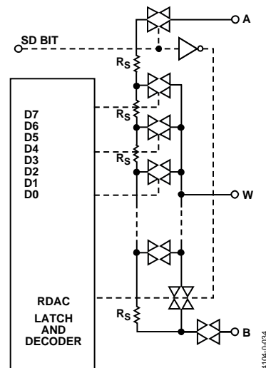
Figure 32. AD5170 Equivalent RDAC Circuit
