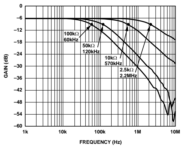
Figure 19. -3 dB Bandwidth @ Code = 0x80
