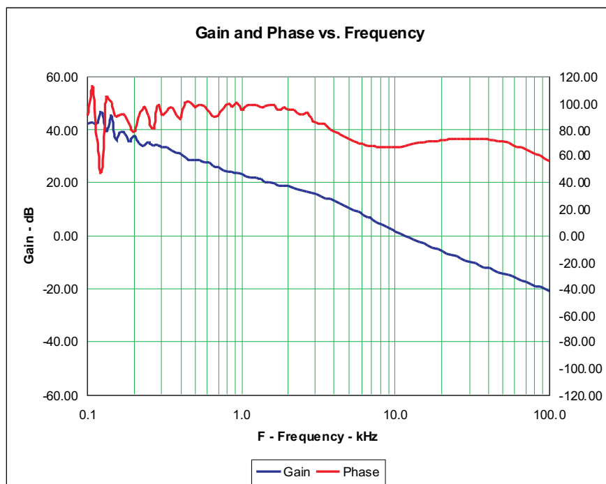
Figure 7. Bode Plots, Test Points Used: TP5 and TP6, ( V_{in} = 48V , I_{o1} = 50mA , I_{o2} = 50mA )
