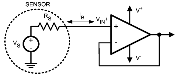
FIGURE 9. Noise Due to I_{BIAS}
