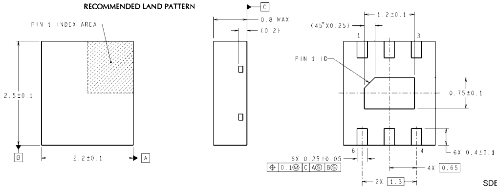
RECOMMENDED LAND PATTERN
